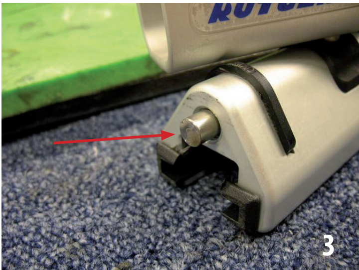
3. When it is out a few millimetres, try to pull it out with a pair of pliers. Change the rubber and mount the axle and the upper part.
